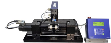
eXpert 9300 - Rotating Beam Fatigue ADMET's Rotating Beam Fatigue Testers feature a dual pivot servo controlled actuator that applies a pure bending moment and is ISO 1143 compliant. Standard models apply moments up to 50Nm at spindle speeds up to 6000RPM . It is ideal for generating S-N curves and evaluating the finite and infinite life of metal samples.
