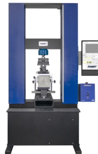
eXpert 2654 - 100kN Dual Column UTM Floor standing machine equipped with ASTM C1609 bend fixture and frame mounted touch panel computer.
