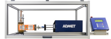
eXpert 5603 - 5kN Single Column UTM Table top machine equipped with custom fixture to peel labels off jars. Frame oriented in horizontal orientation with safety cage.
